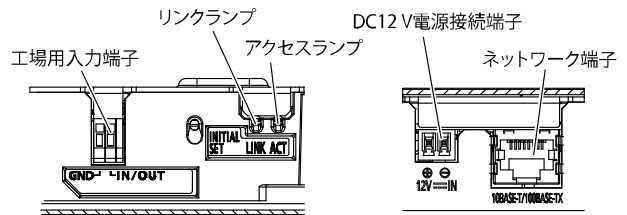
矢視図A
