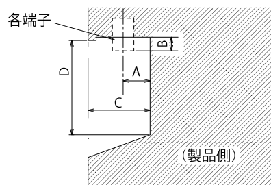
端子部 b 断面 (IR OUT/SERIAL OUT/AUDIO OUT/IR IN/SERIAL IN/AV IN)
